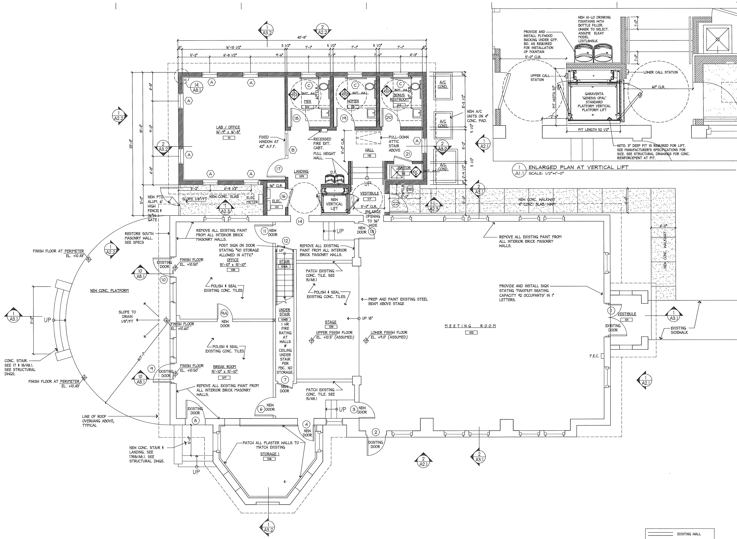
1 PROPOSED FIRST FLOOR PLAN A1.1 SCALE: 1/4"=1'-0"
